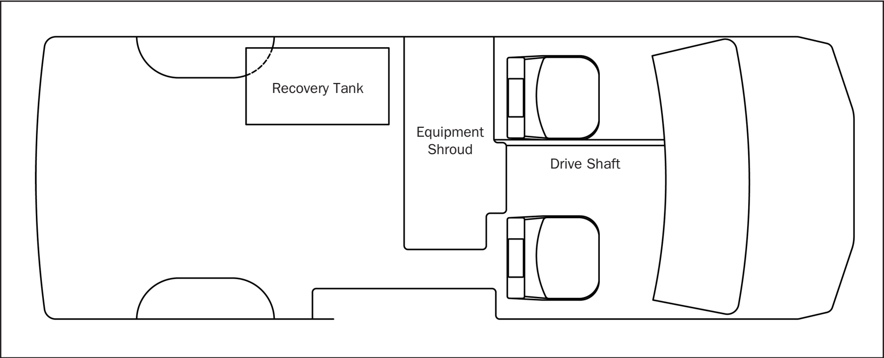
Floor plan is to exact scale in a Standard Length Van.
